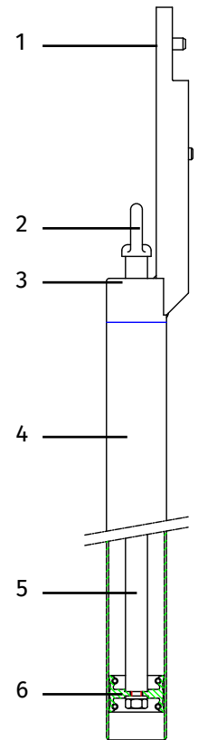
Piston sampler
